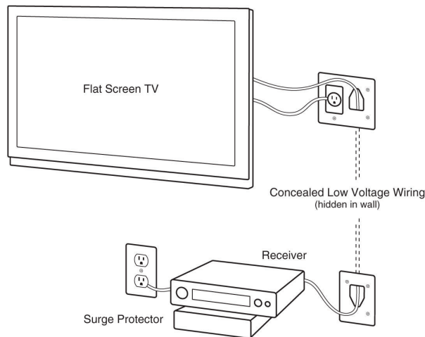
Front View- Installation Diagram
