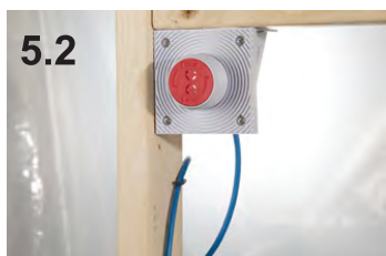
Figure 5.1 & 5.2: Make a loop with your prewire, run it through the RDM threaded insert opening, and wire tie the loop to the back of the RED mud shield. Then insert the RED mud shield into the RDM threaded insert, and turn clockwise to lock it in place. You may need to hold the threaded insert to keep it from spinning. You are now ready to install the wall finish.
